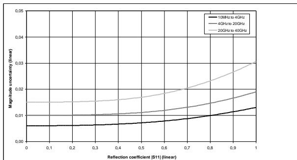
Typical accuracy of reflection magnitude and reflection phase measurements for the R&S®ZNB40 model .72 in the frequency range from 10 MHz to 40 GHz. Analysis conditions: S_{12} = S_{21} = 0 , cal. power -10 dBm, meas. power -10 dBm.
