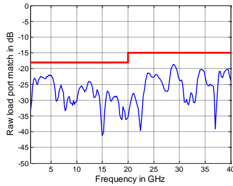
Raw load port match versus frequency for the R&S®ZNB40 model .82 and .84.
