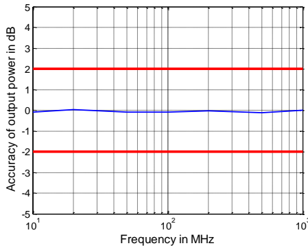
Output power accuracy in dB versus frequency for the R&S®ZNB40 model .72.
