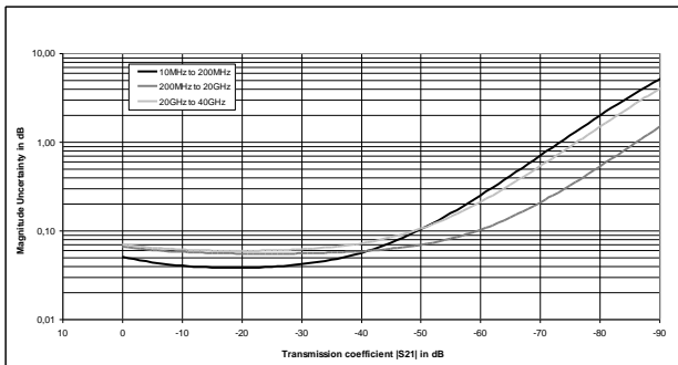
Typical accuracy of transmission magnitude and transmission phase measurements for the R&S®ZNB40 model .72 in the frequency range from 10 MHz to 40 GHz. Analysis conditions: S_{11} = S_{22} = 0 , cal. power -10 dBm, meas. power -10 dBm.
