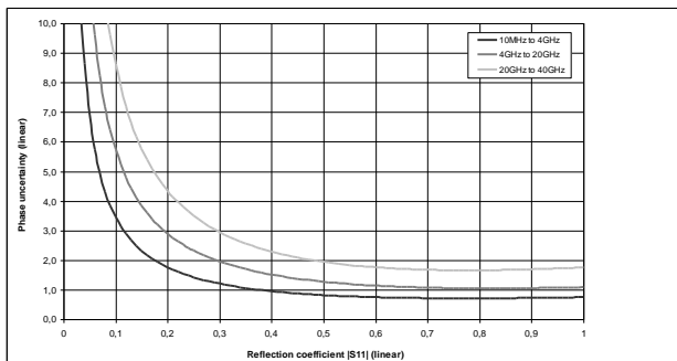
Typical accuracy of reflection magnitude and reflection phase measurements for the R&S®ZNB40 model .72 in the frequency range from 10 MHz to 40 GHz. Analysis conditions: S_{12} = S_{21} = 0 , cal. power -10 dBm, meas. power -10 dBm.
