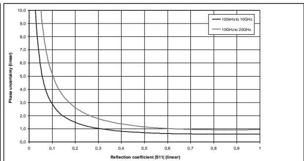
Typical accuracy of reflection magnitude and reflection phase measurements for the R&S®ZNB20 in the frequency range from 100 kHz to 20 GHz. Analysis conditions: S_{12} = S_{21} = 0 , cal. power -10 dBm, meas. power -10 dBm.
