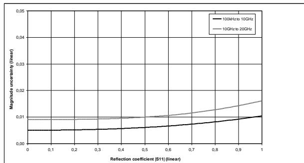
Typical accuracy of reflection magnitude and reflection phase measurements for the R&S®ZNB20 in the frequency range from 100 kHz to 20 GHz. Analysis conditions: S_{12} = S_{21} = 0 , cal. power -10 dBm, meas. power -10 dBm.
