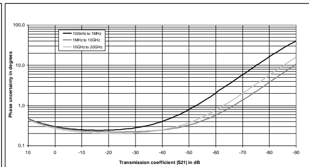
Typical accuracy of transmission magnitude and transmission phase measurements for the R&S®ZNB20 in the frequency range from 100 kHz to 20 GHz. Analysis conditions: S_{11} = S_{22} = 0 , cal. power -10 dBm, meas. power -10 dBm.
