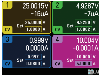
Figure 2. In Meter View, all 4 outputs can be viewed simultaneously. The both measured values for voltage and current are displayed for each output.
